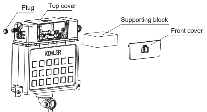
In-Wall Tank Without Frame on timber
