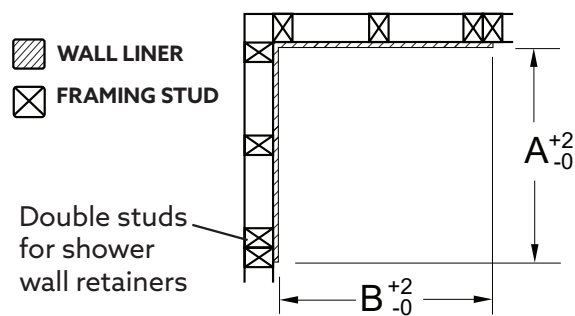
Fig. 3: Recommended Timber Frame for Shower Enclosure Installation
