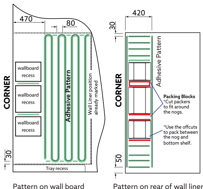
Fig.13: Adhesive pattern for Side Recessed Walls
