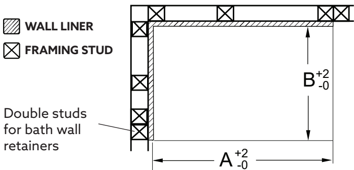
Fig. 2: Recommended BATH Timber Frame for Shower Enclosure Installation
