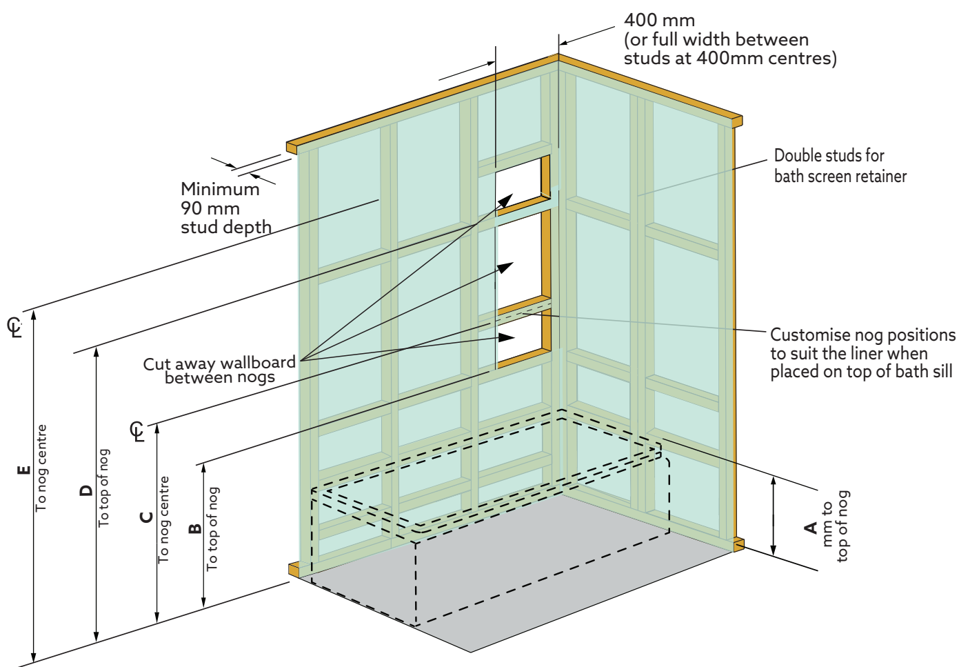
Fig. 5b: Framing and Wallboard Preparation for Side Recessed Bath Wall Liners
