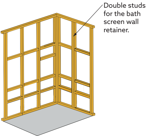
Fig. 2: Recommended BATH Timber Frame for Shower Enclosure Installation
