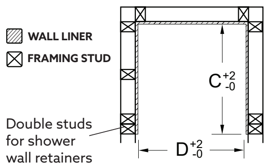
Fig1 : Alcove (3 sided) Wall
