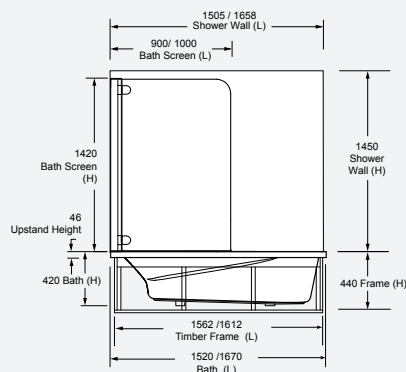
DROP-IN BATH WITH FLAT PACK FRAME INSTALLED
