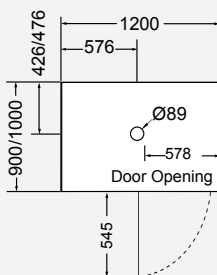
1200 x 900 / 1200 x 1000 RIGHT HAND
