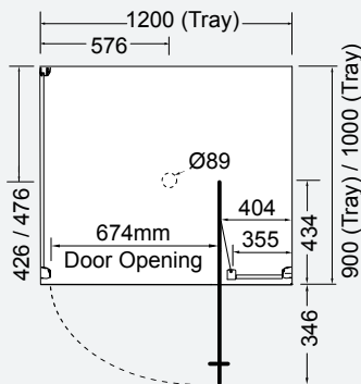
1200 x 900 / 1200 x 1000 CENTRE WASTE, LEFT HAND
