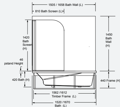
DROP-IN BATH WITH FLAT PACK FRAME INSTALLED
