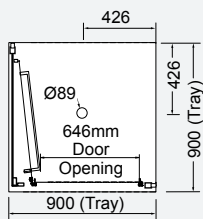
900 x 900 CENTRE WASTE
