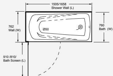
BATH SCREEN OPEN
