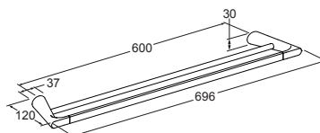
Valencia Double Towel Rail - 75810A-CP
