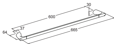
Valencia Single Towel Rail - 75809A-CP
