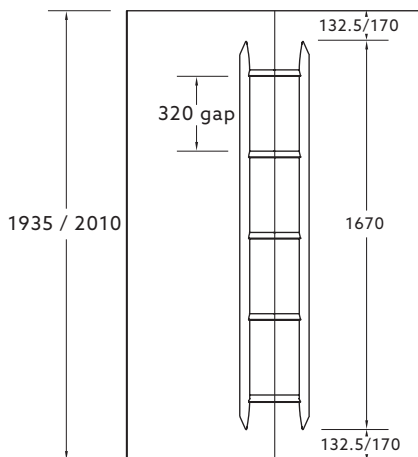
Front View (Generic)
