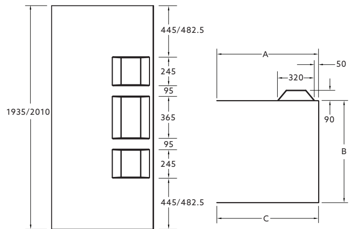
Section View (Generic - 3 sided)
