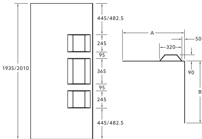
Front View (Generic - 2 sided)
