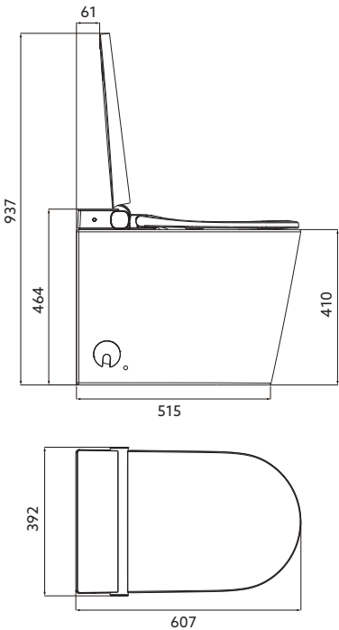
Rough-In (in mm)
