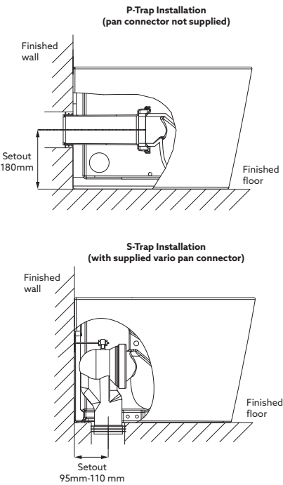
Set-Out
