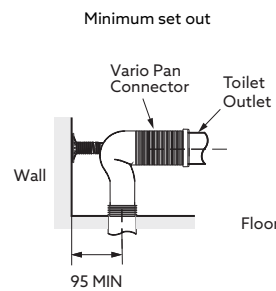
Vario Standard Pan Connector (SKU#: 1534531) S-trap Installation
